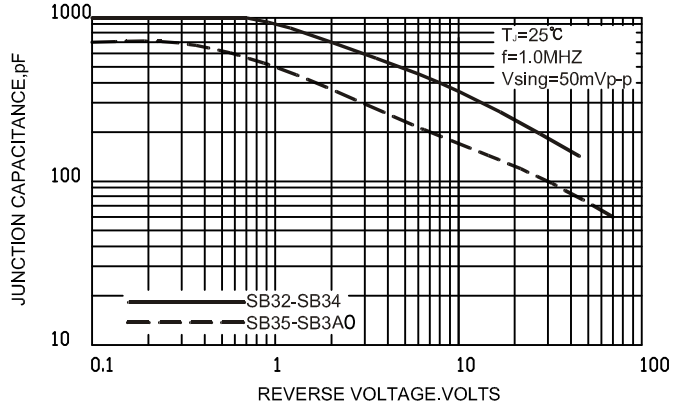
FIG.5-TYPICAL JUNCTION CAPACITANCE
